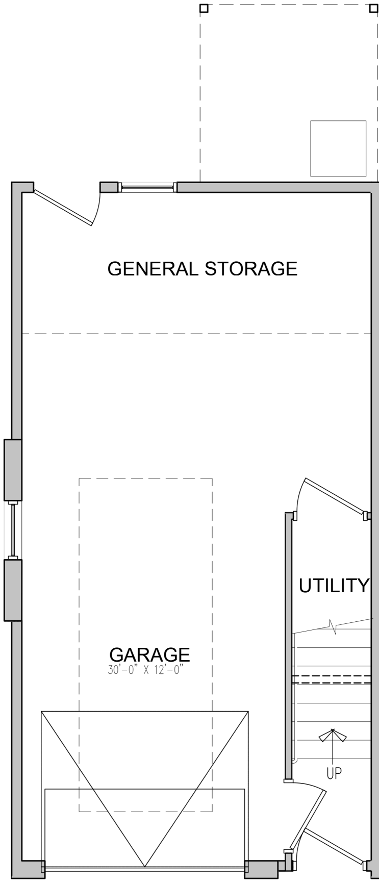
GROUND FLOOR
