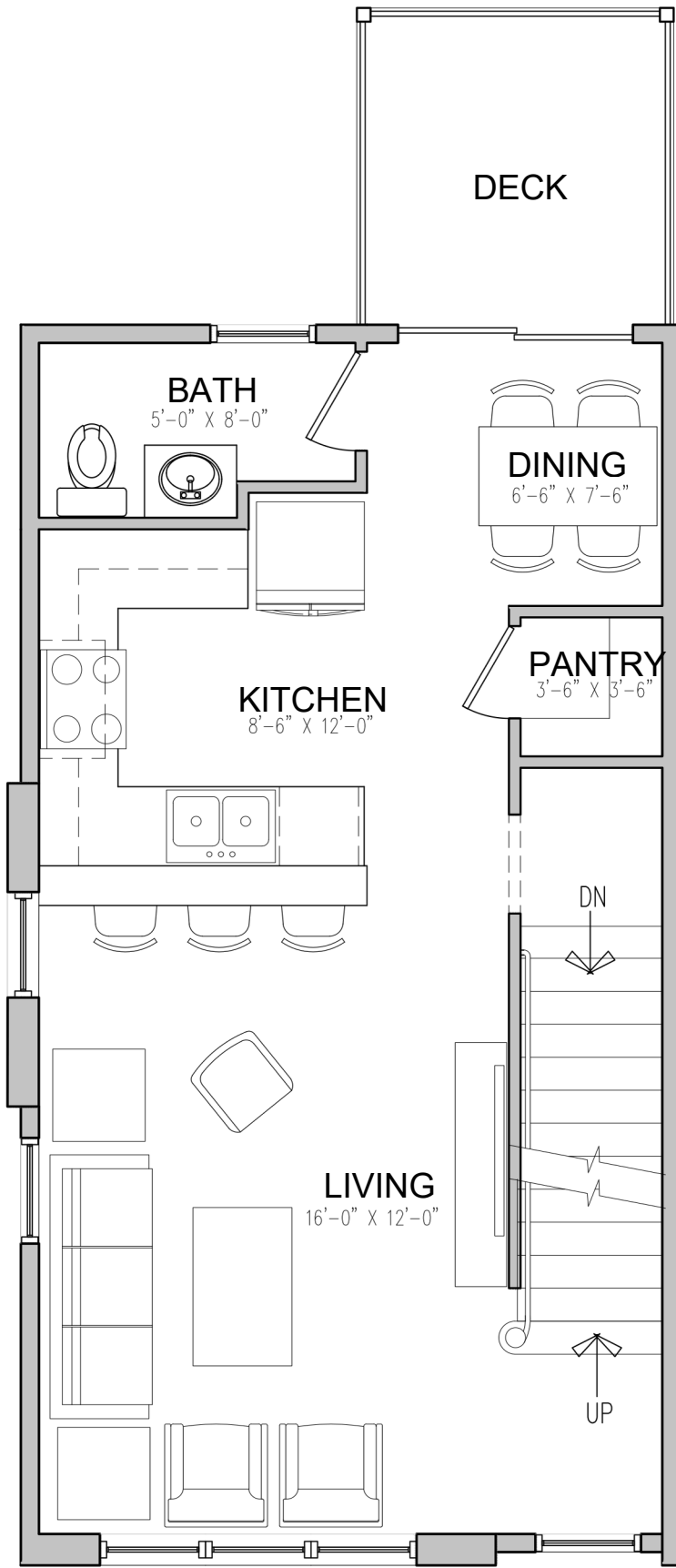
FIRST FLOOR
